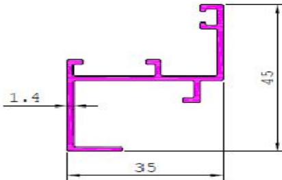
S3298 0.921 kg/m
