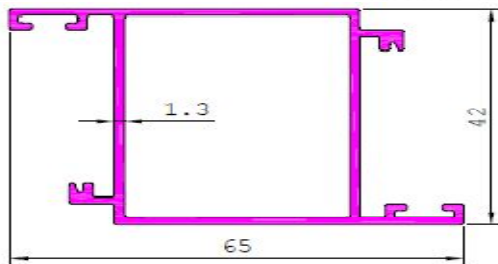
S3167 0.776 kg/m
