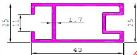
20518 0.675 kg/m
